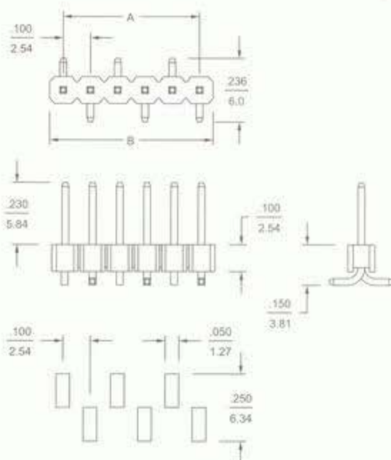
P. C. board hole dimensions
