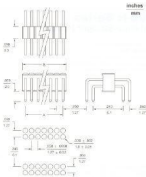
F.C. board hole dimensions
